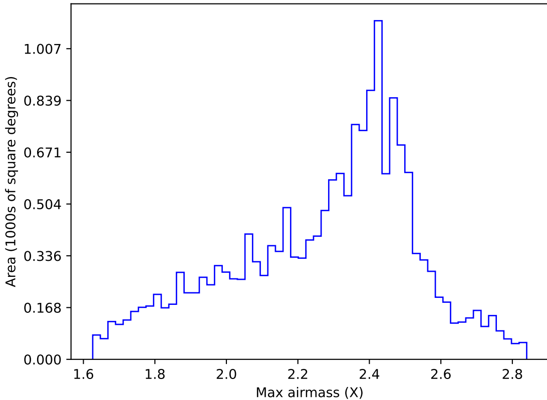
too_ignore_100_1v3.4_10yrs WFD r band: Max airmass
