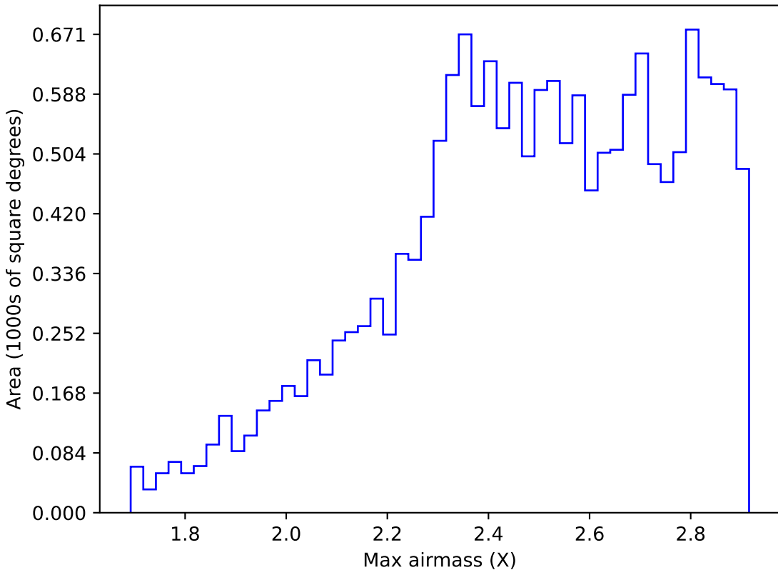
too_ignore_100_1v3.4_10yrs WFD i band: Max airmass
