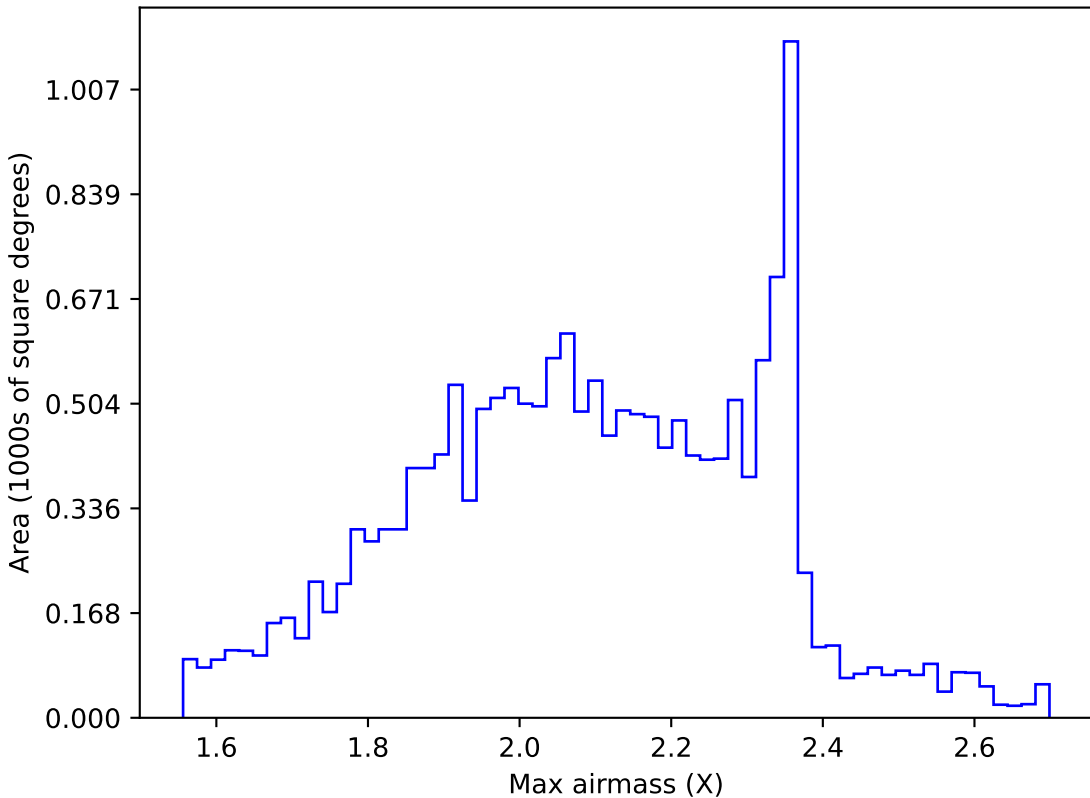
too_ignore_100_1v3.4_10yrs WFD g band: Max airmass
