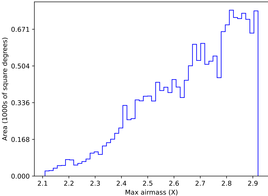
too_ignore_100_1v3.4_10yrs WFD all bands: Max airmass
