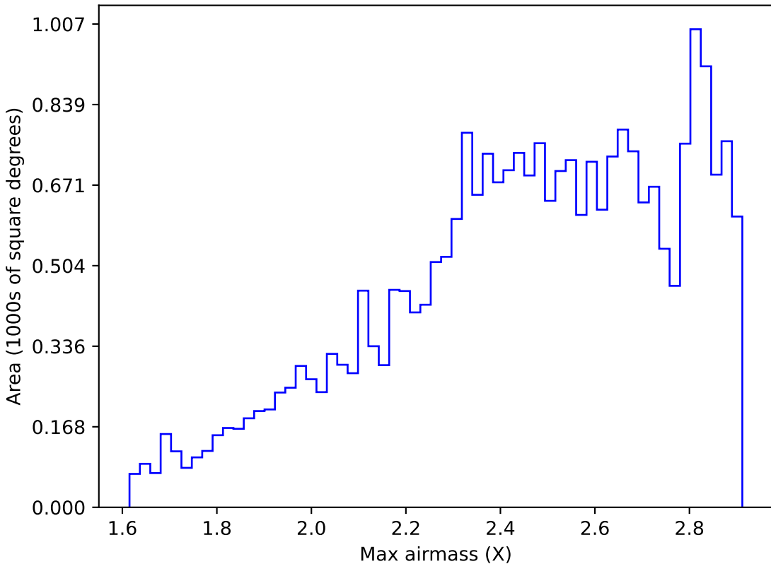
too_ignore_100_1v3.4_10yrs All sky z band: Max airmass
