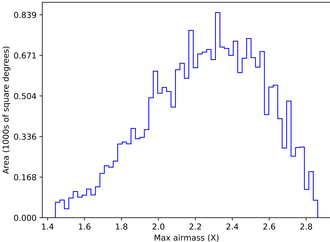
too_ignore_100_1v3.4_10yrs All sky y band: Max airmass
