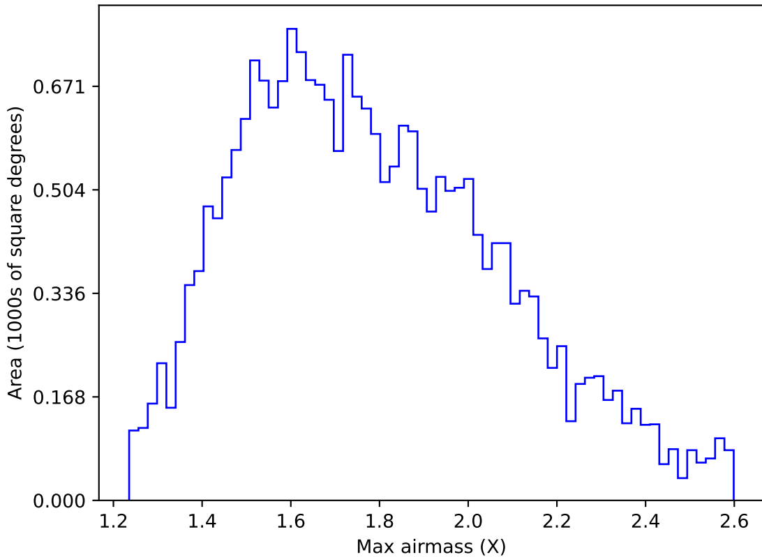
too_ignore_100_1v3.4_10yrs All sky u band: Max airmass
