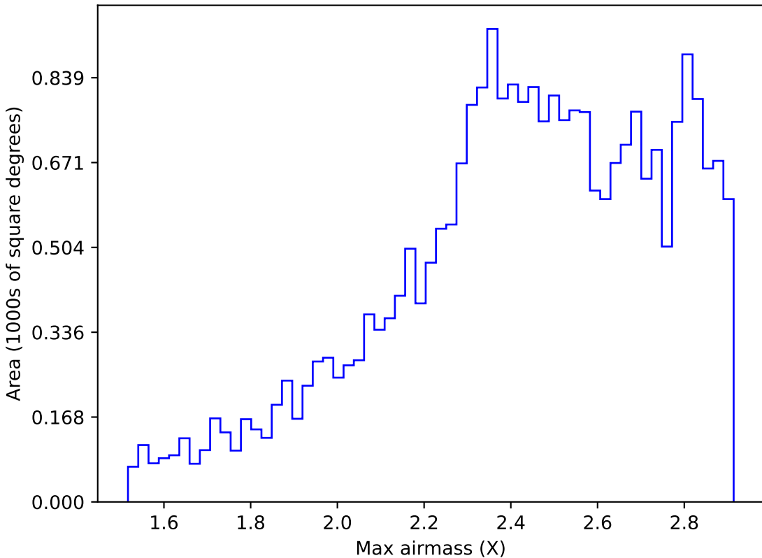
too_ignore_100_1v3.4_10yrs All sky i band: Max airmass
