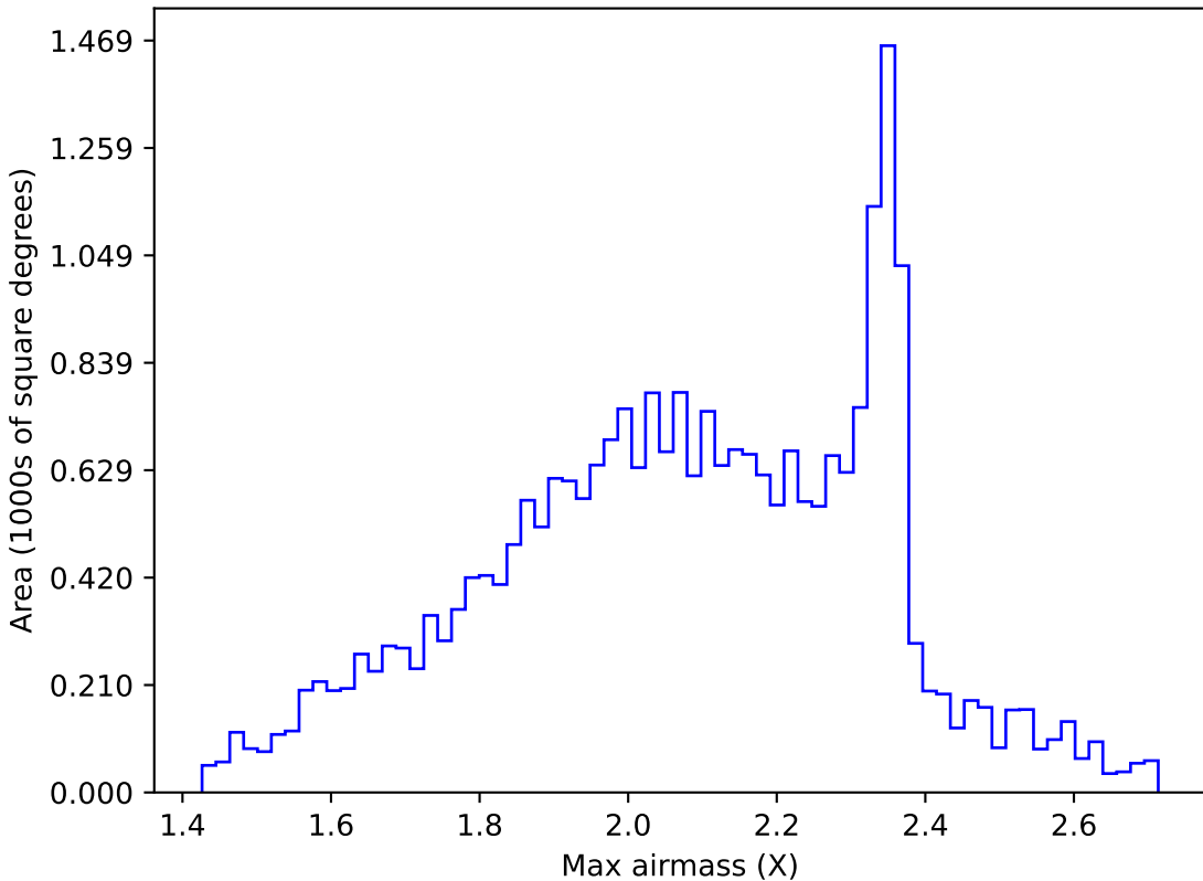
too_ignore_100_1v3.4_10yrs All sky g band: Max airmass
