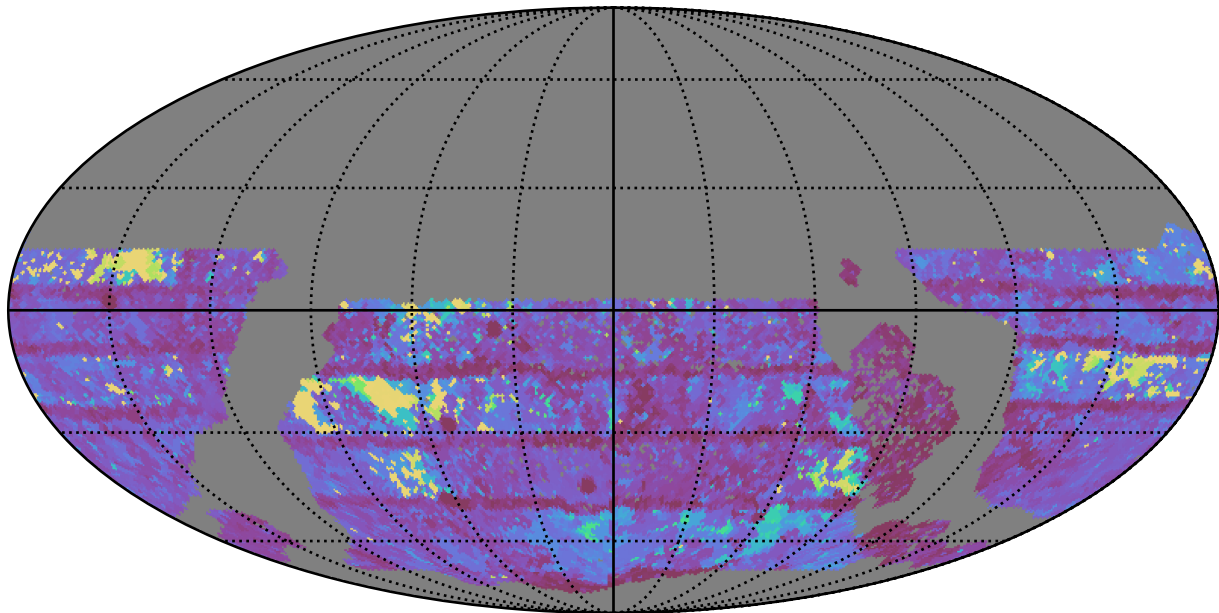
too_ignore_100_1v3.4_10yrs WFD z band: Max Inter-Night Gap
