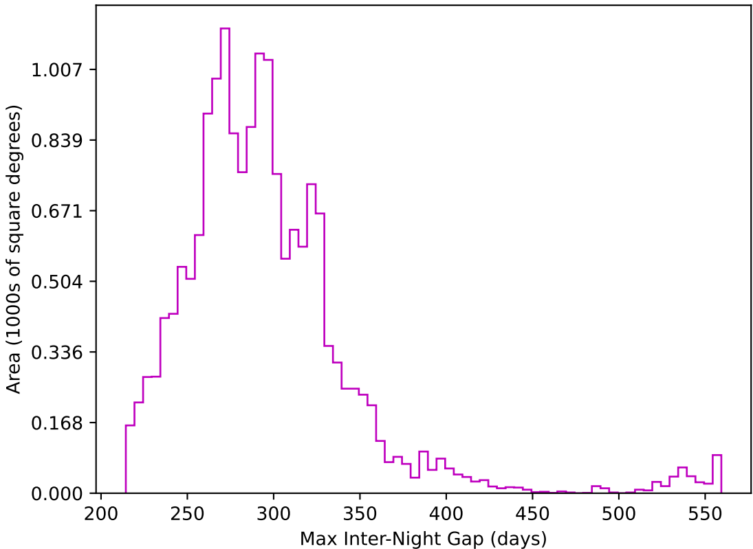
too_ignore_100_1v3.4_10yrs WFD z band: Max Inter-Night Gap
