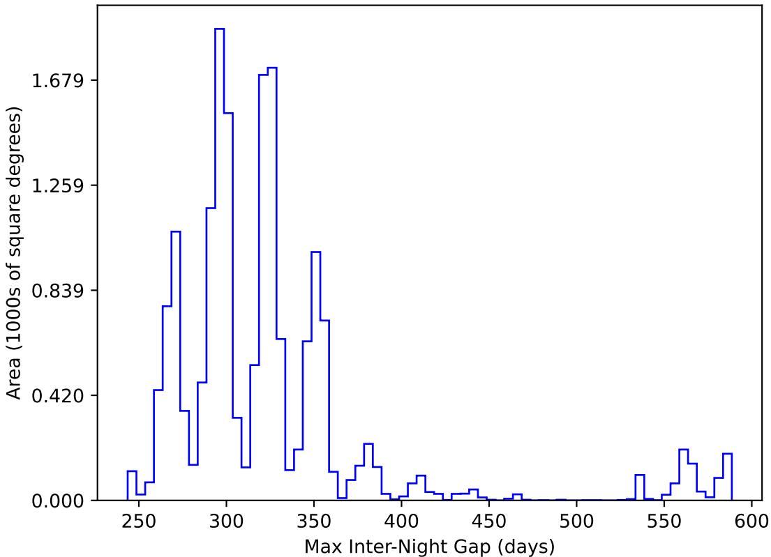
too_ignore_100_1v3.4_10yrs WFD y band: Max Inter-Night Gap
