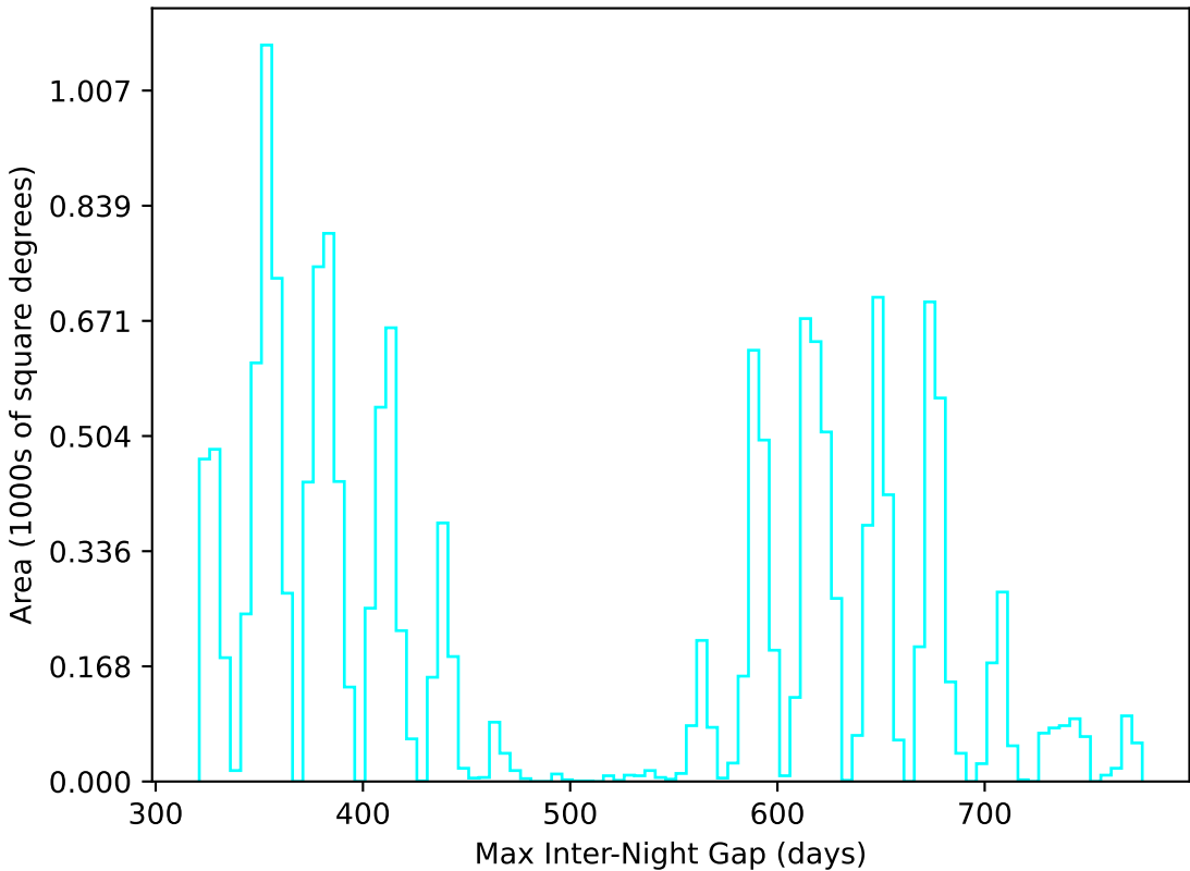
too_ignore_100_1v3.4_10yrs WFD u band: Max Inter-Night Gap
