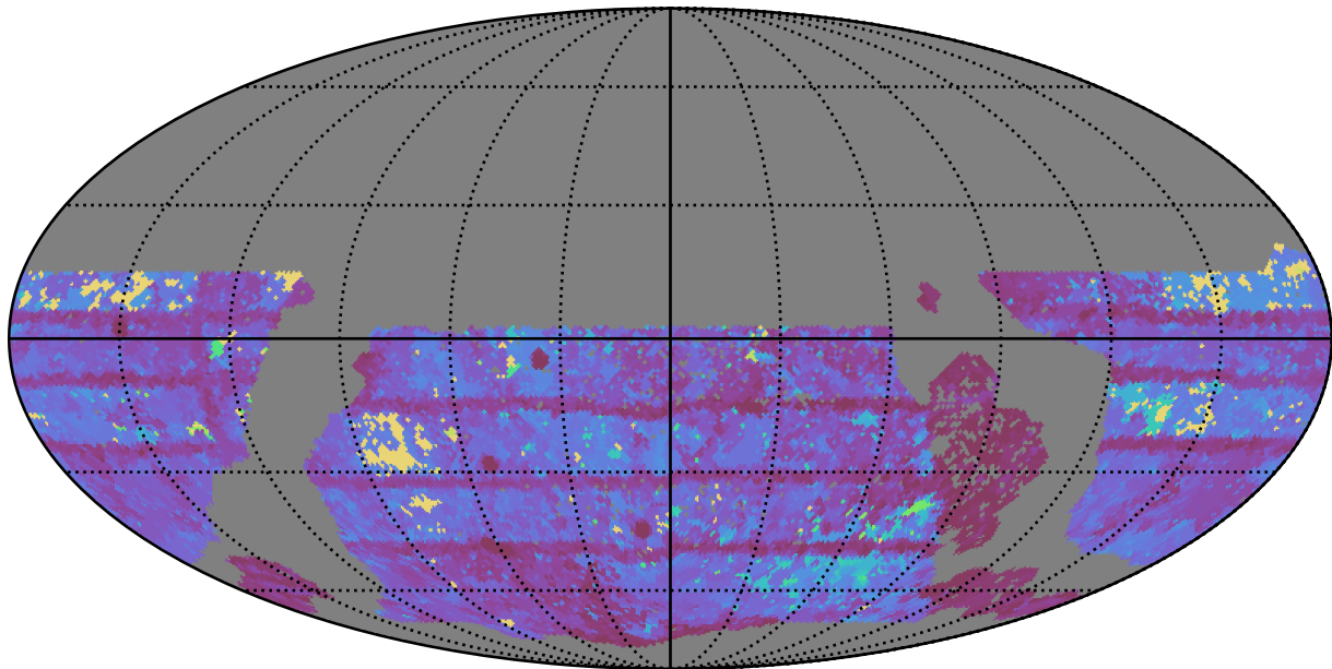
too_ignore_100_1v3.4_10yrs WFD r band: Max Inter-Night Gap
