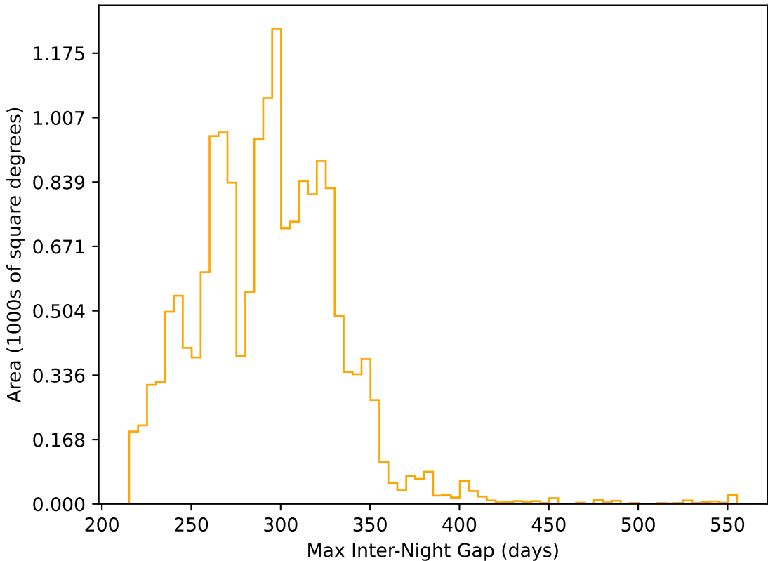
too_ignore_100_1v3.4_10yrs WFD r band: Max Inter-Night Gap
