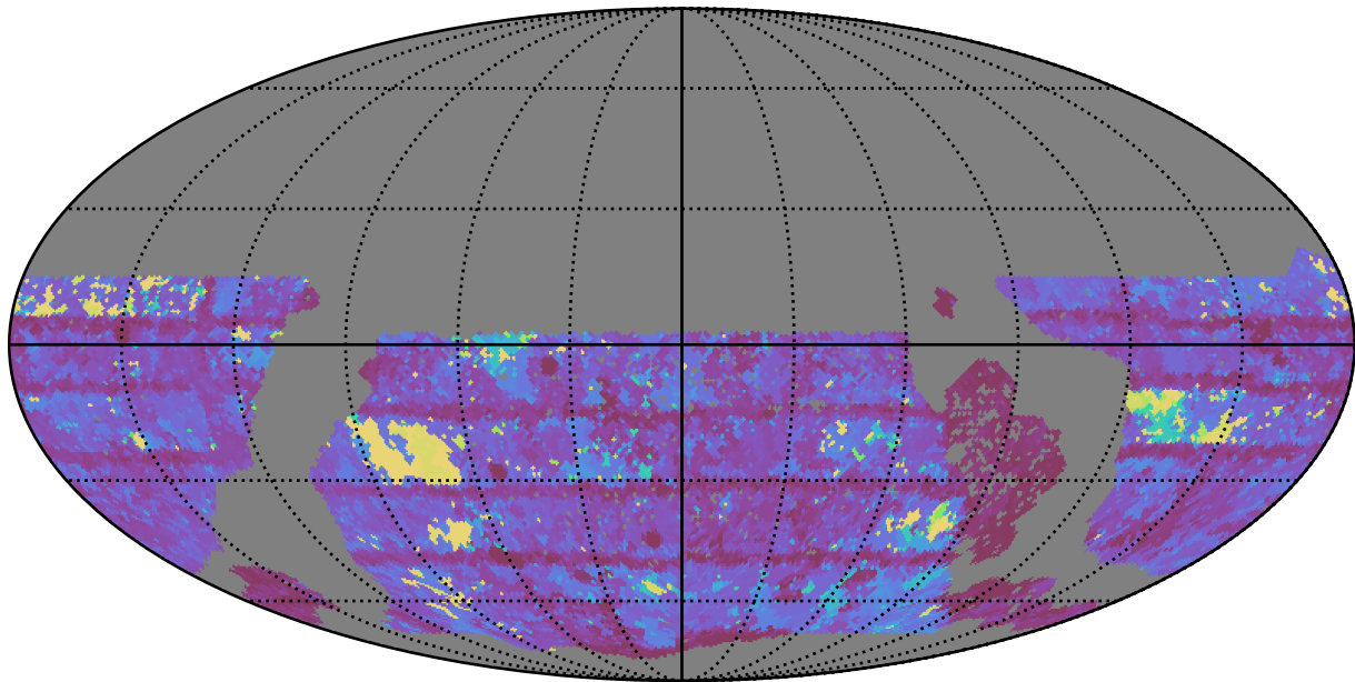
too_ignore_100_1v3.4_10yrs WFD i band: Max Inter-Night Gap
