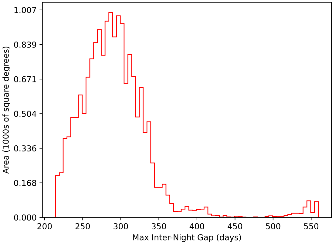
too_ignore_100_1v3.4_10yrs WFD i band: Max Inter-Night Gap
