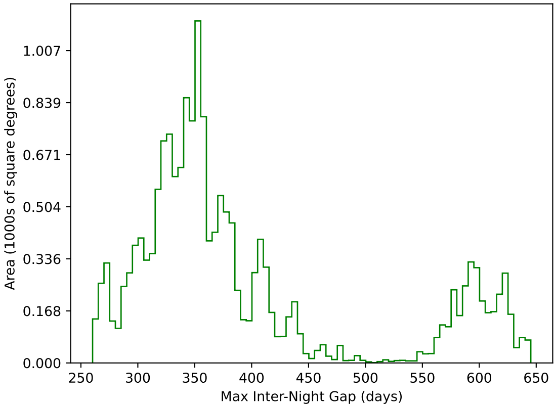
too_ignore_100_1v3.4_10yrs WFD g band: Max Inter-Night Gap
