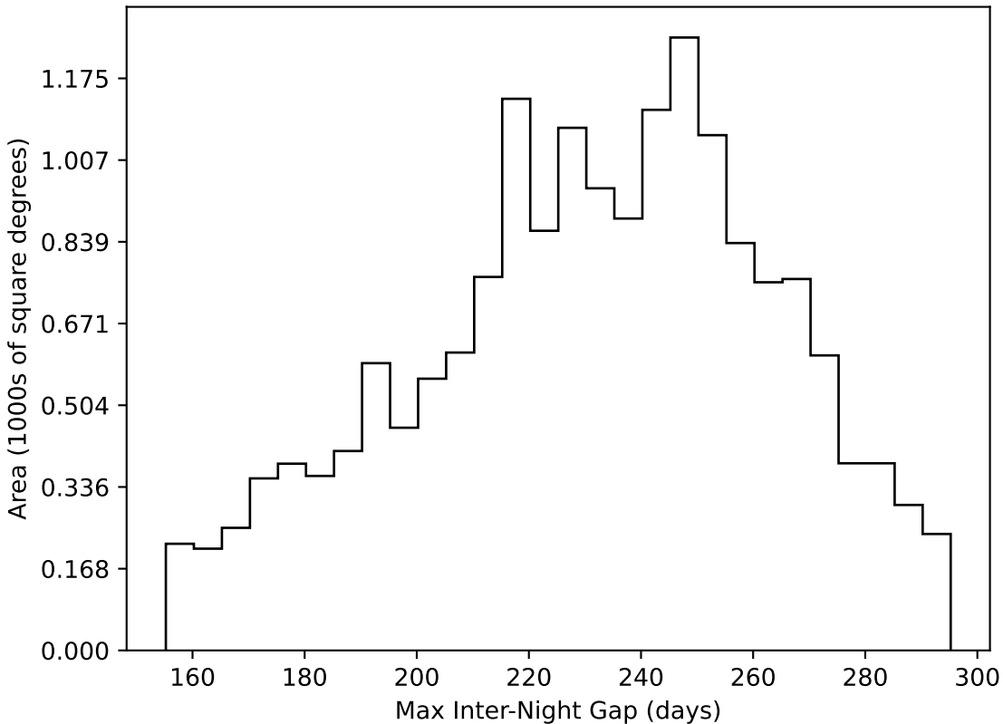
too_ignore_100_1v3.4_10yrs WFD all bands: Max Inter-Night Gap
