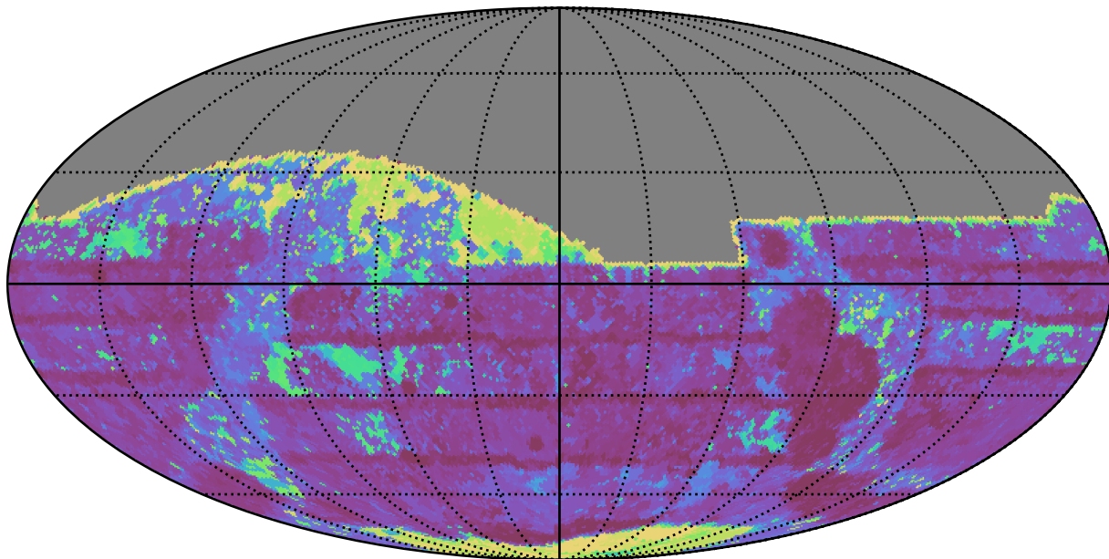
too_ignore_100_1v3.4_10yrs All sky z band: Max Inter-Night Gap
