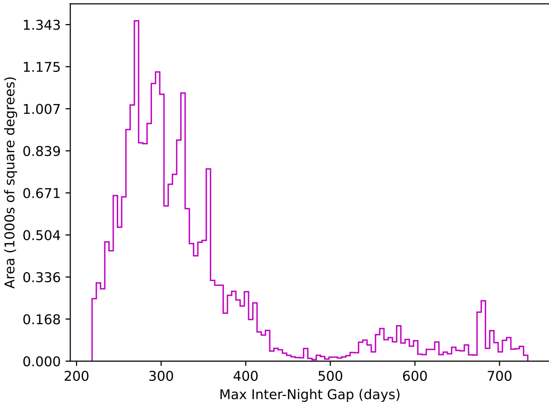
too_ignore_100_1v3.4_10yrs All sky z band: Max Inter-Night Gap
