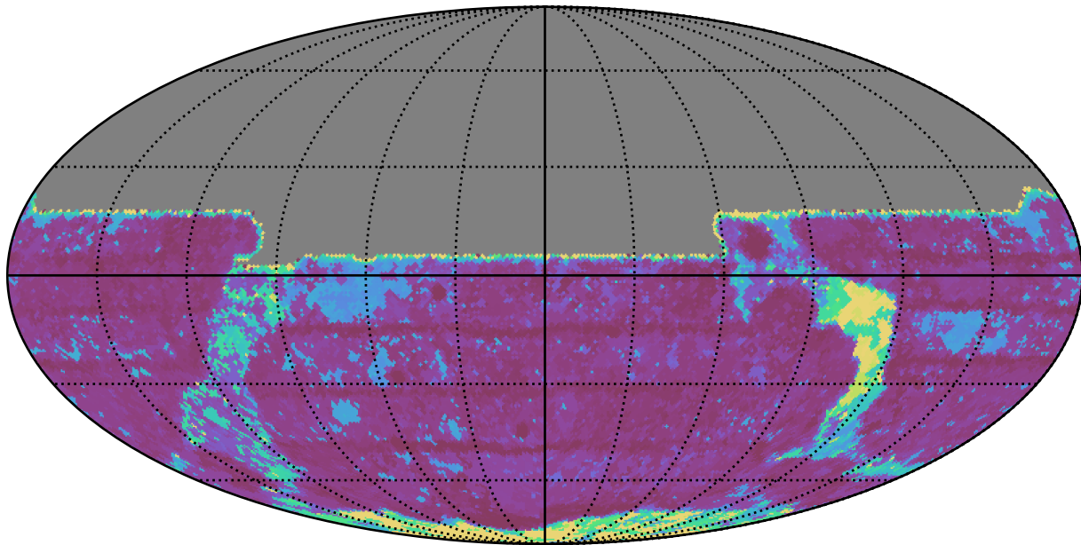
too_ignore_100_1v3.4_10yrs All sky y band: Max Inter-Night Gap
