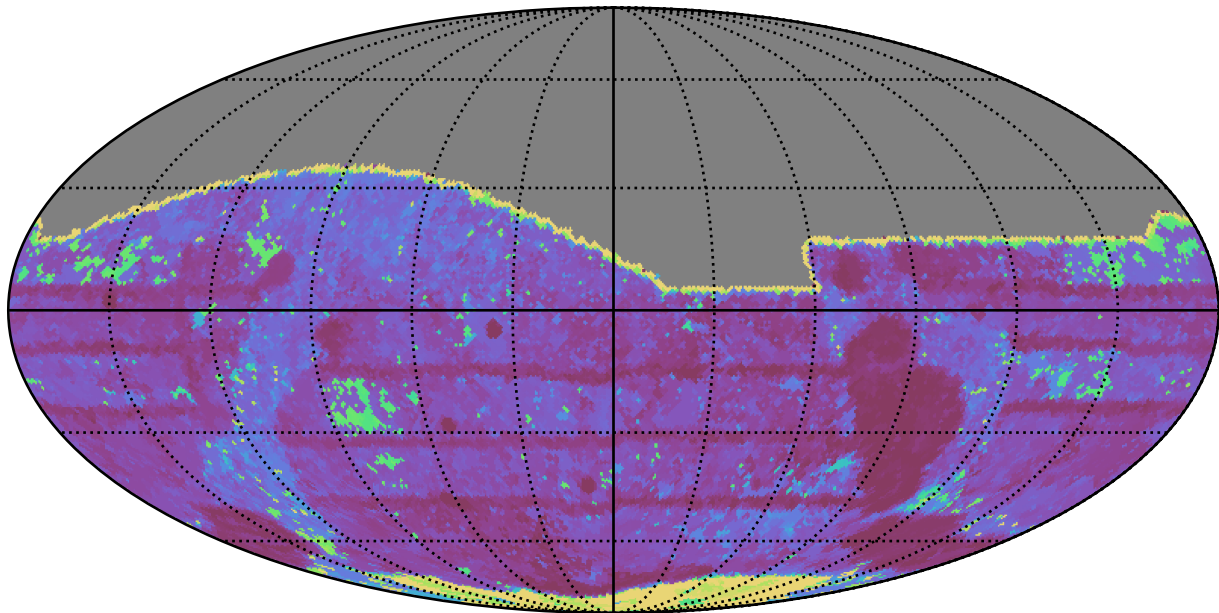
too_ignore_100_1v3.4_10yrs All sky r band: Max Inter-Night Gap
