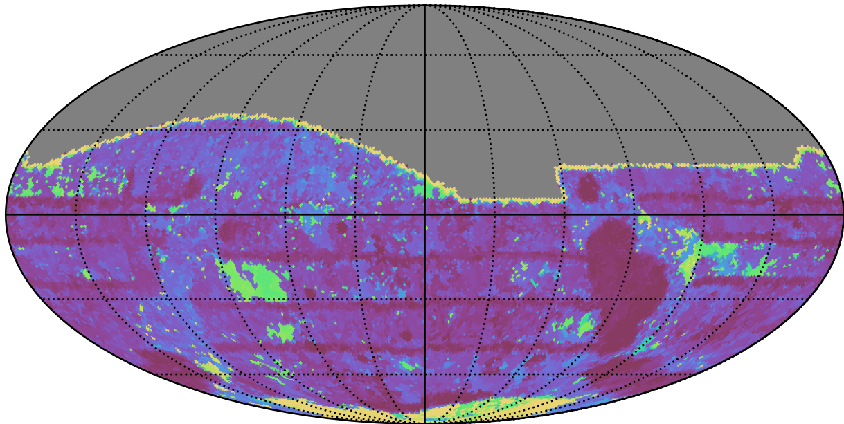
too_ignore_100_1v3.4_10yrs All sky i band: Max Inter-Night Gap
