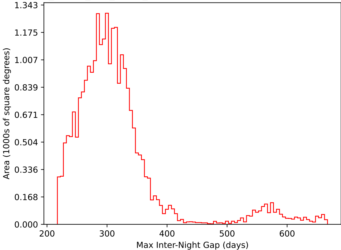
too_ignore_100_1v3.4_10yrs All sky i band: Max Inter-Night Gap
