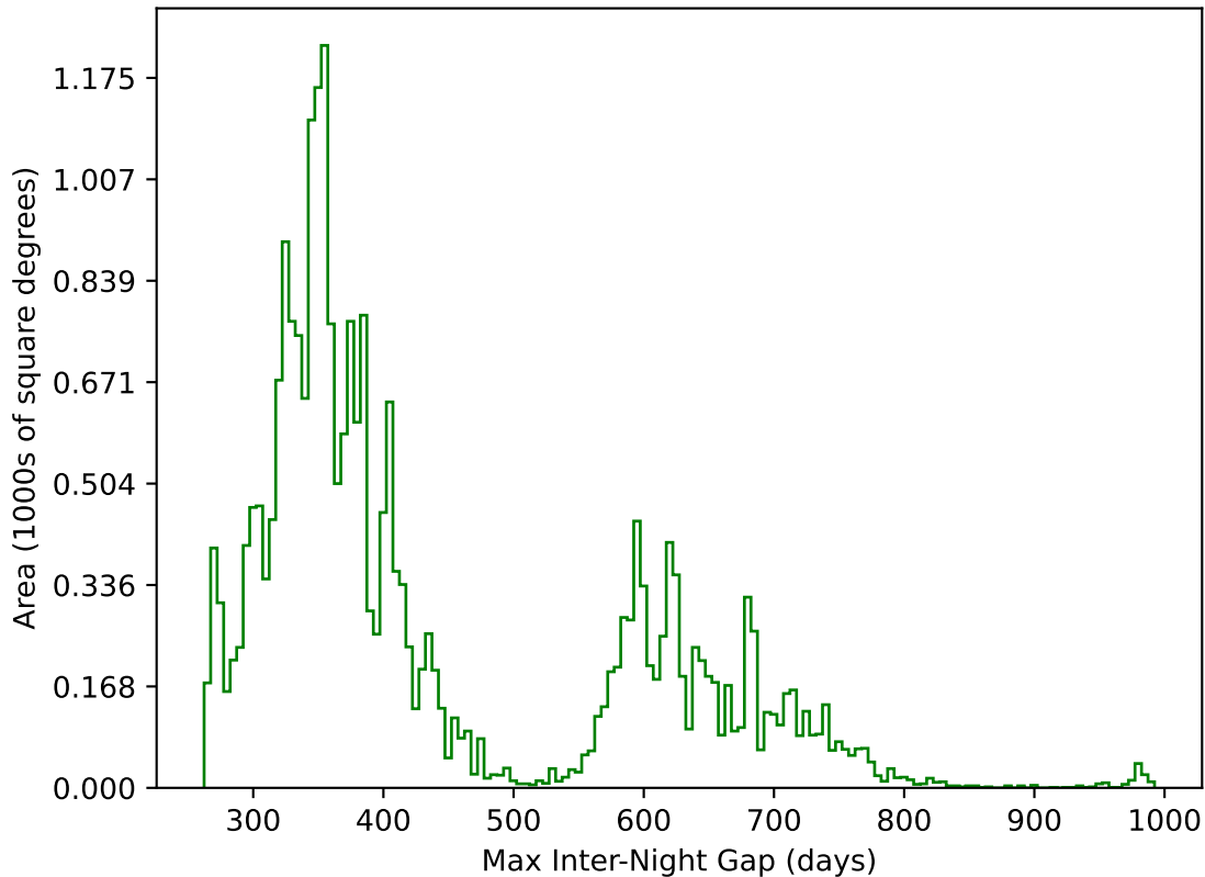
too_ignore_100_1v3.4_10yrs All sky g band: Max Inter-Night Gap
