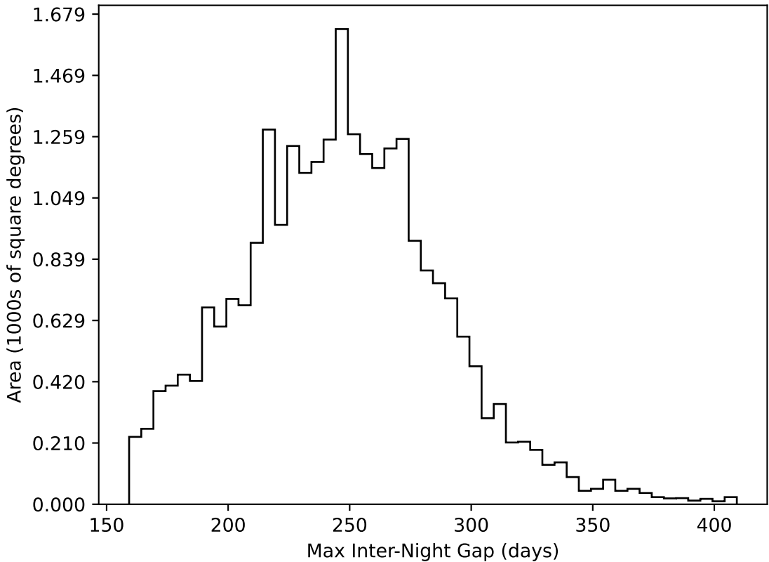
too_ignore_100_1v3.4_10yrs All sky all bands: Max Inter-Night Gap
