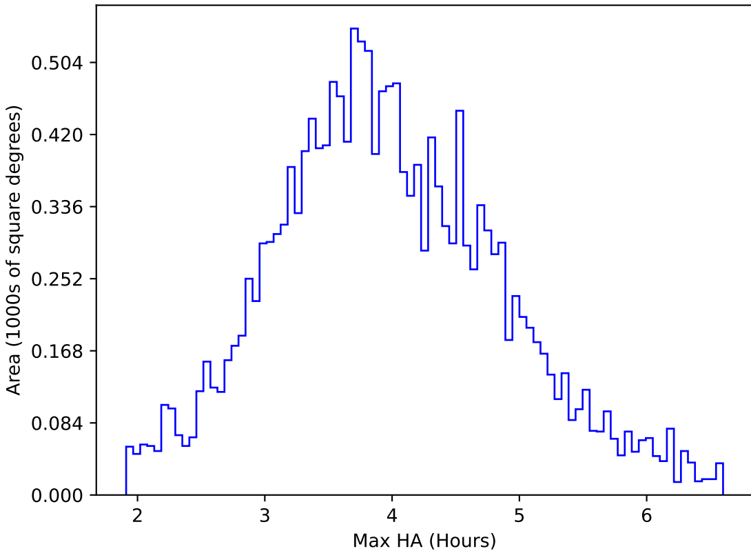
too_ignore_100_1v3.4_10yrs WFD u band: Max HA
