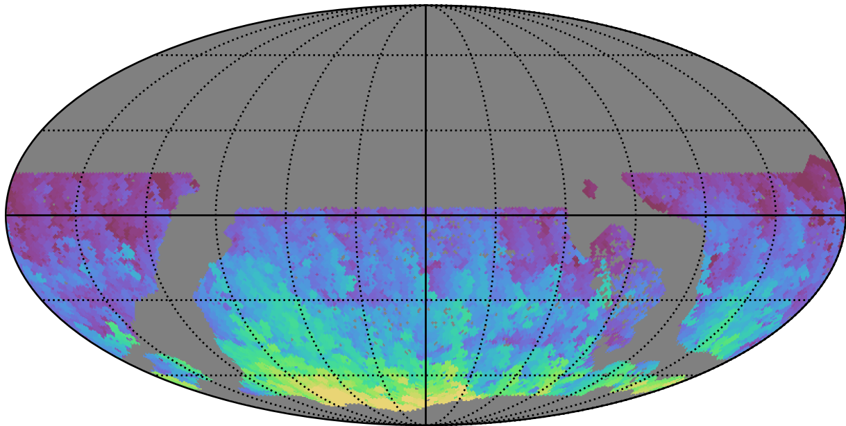
too_ignore_100_1v3.4_10yrs WFD r band: Max HA
