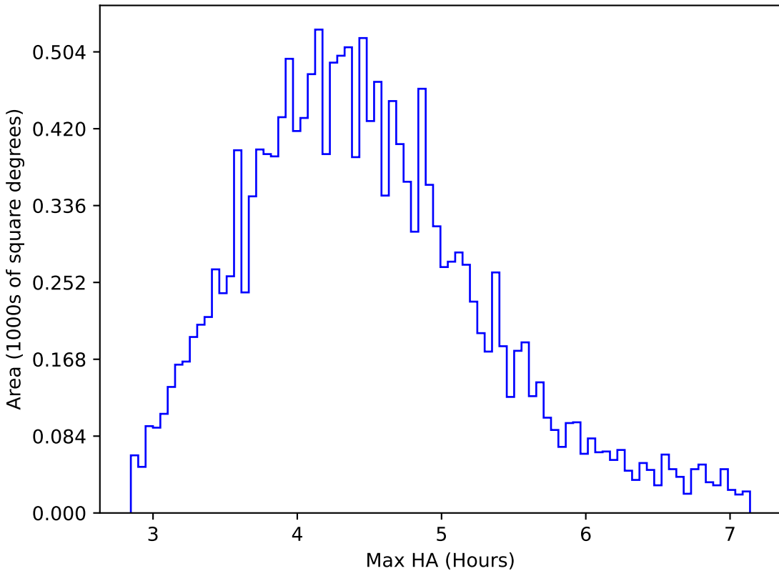
too_ignore_100_1v3.4_10yrs WFD r band: Max HA
