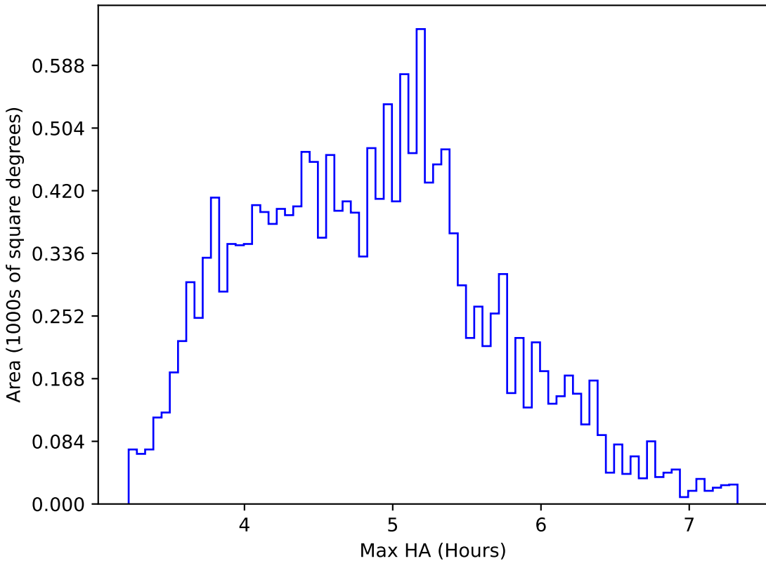
too_ignore_100_1v3.4_10yrs WFD i band: Max HA
