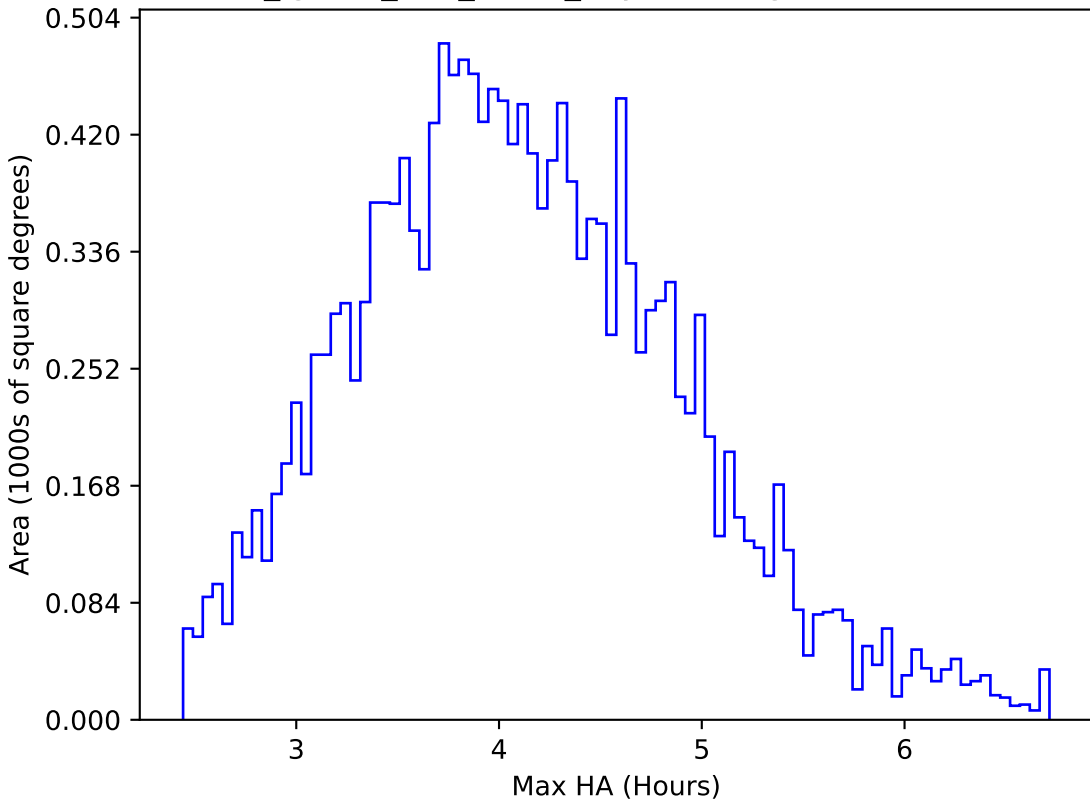
too_ignore_100_1v3.4_10yrs WFD g band: Max HA
