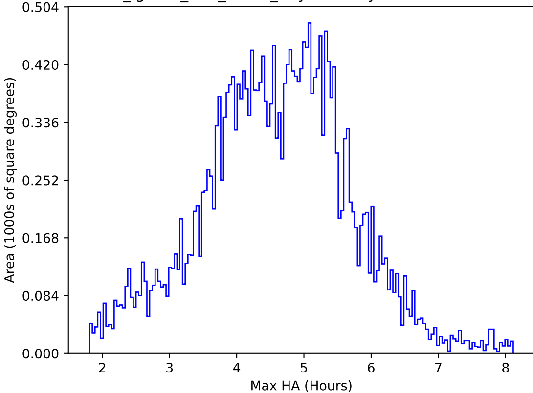
too_ignore_100_1v3.4_10yrs All sky z band: Max HA
