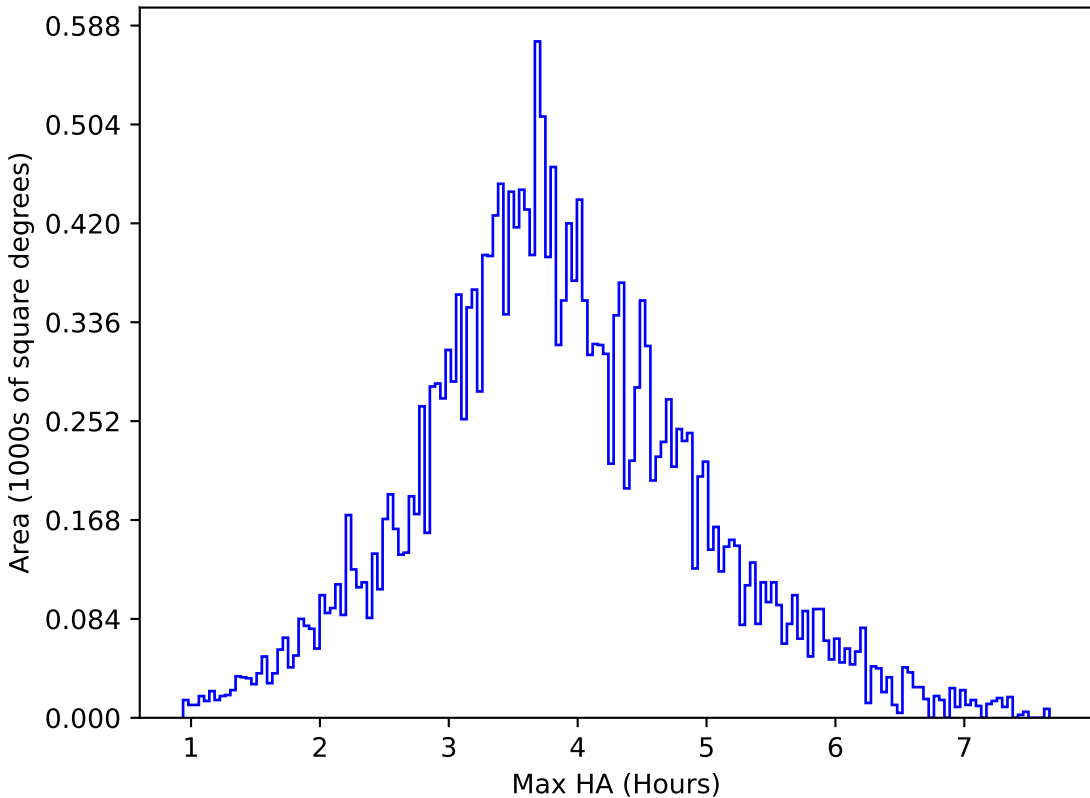
too_ignore_100_1v3.4_10yrs All sky u band: Max HA
