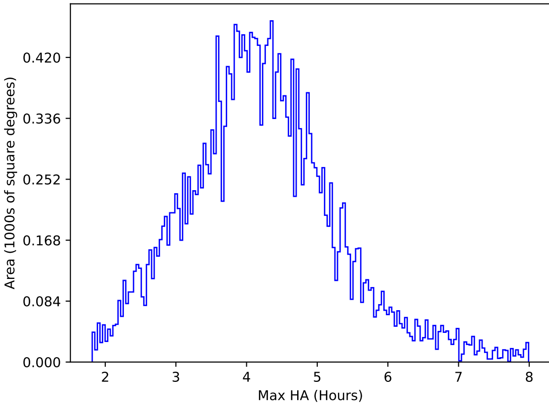
too_ignore_100_1v3.4_10yrs All sky r band: Max HA
