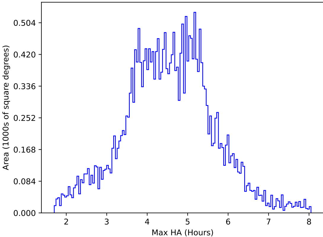
too_ignore_100_1v3.4_10yrs All sky i band: Max HA
