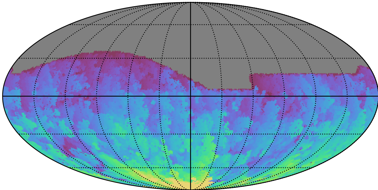
too_ignore_100_1v3.4_10yrs All sky g band: Max HA
