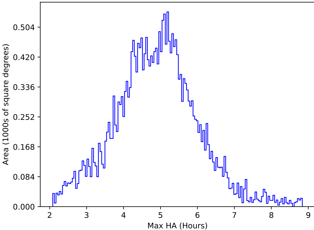
too_ignore_100_1v3.4_10yrs All sky all bands: Max HA
