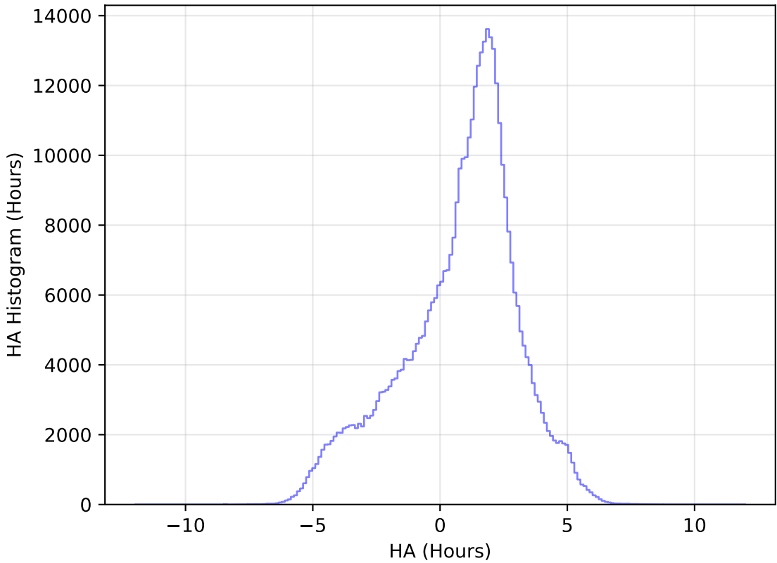
too_ignore_100_1v3.4_10yrs WFD z band: HA Histogram
