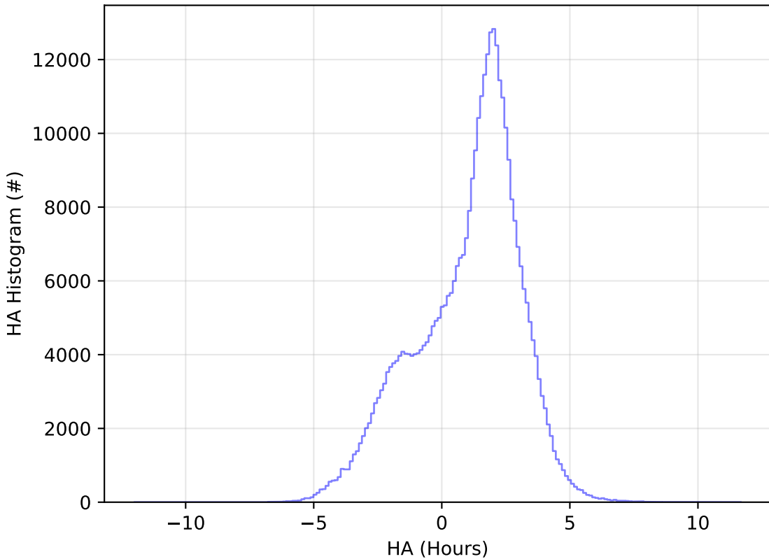
too_ignore_100_1v3.4_10yrs WFD y band: HA Histogram
