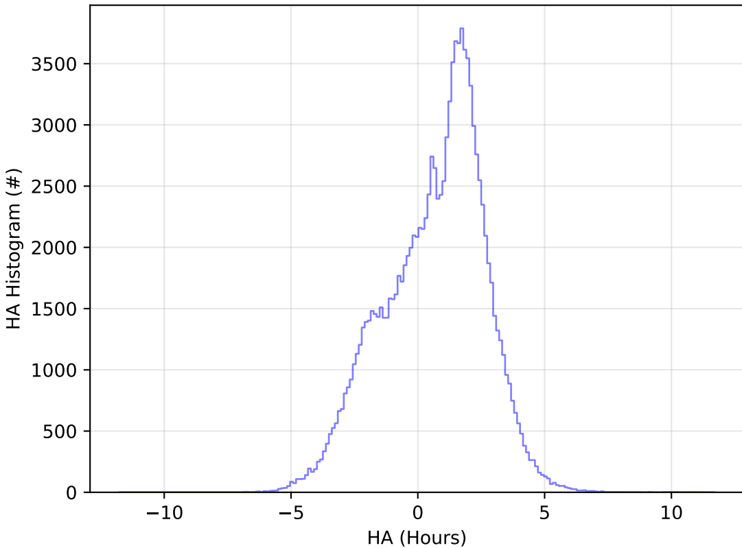
too_ignore_100_1v3.4_10yrs WFD u band: HA Histogram
