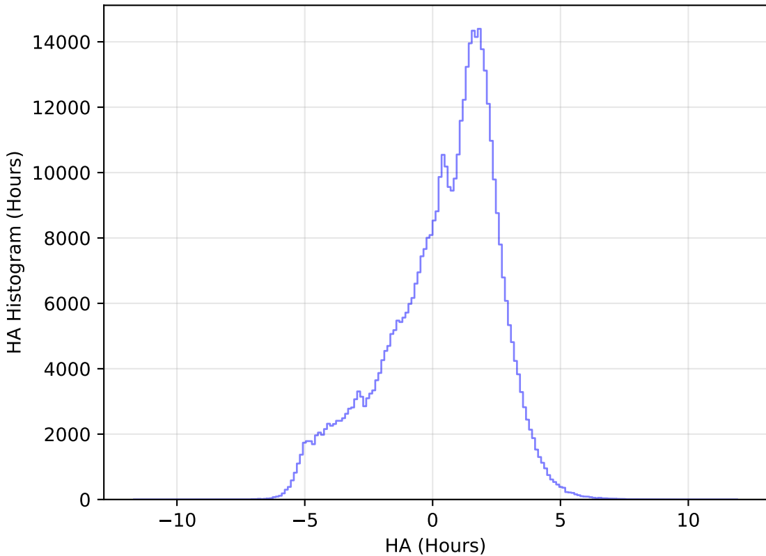
too_ignore_100_1v3.4_10yrs WFD r band: HA Histogram
