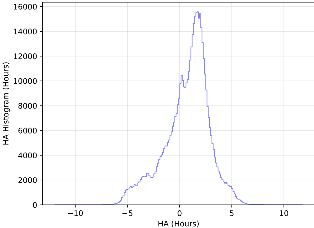
too_ignore_100_1v3.4_10yrs WFD i band: HA Histogram
