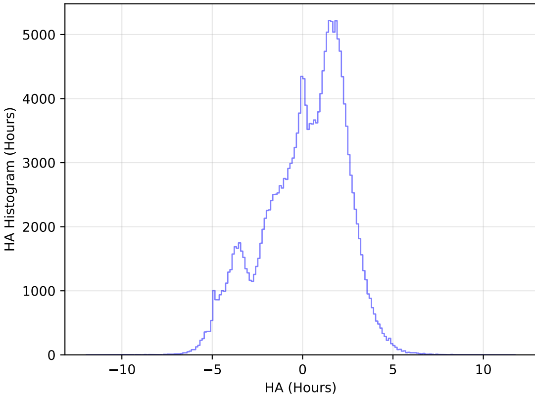
too_ignore_100_1v3.4_10yrs WFD g band: HA Histogram
