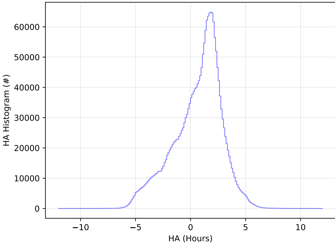
too_ignore_100_1v3.4_10yrs WFD all bands: HA Histogram
