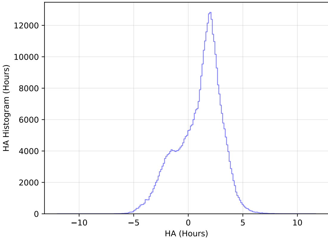
too_ignore_100_1v3.4_10yrs All sky y band: HA Histogram
