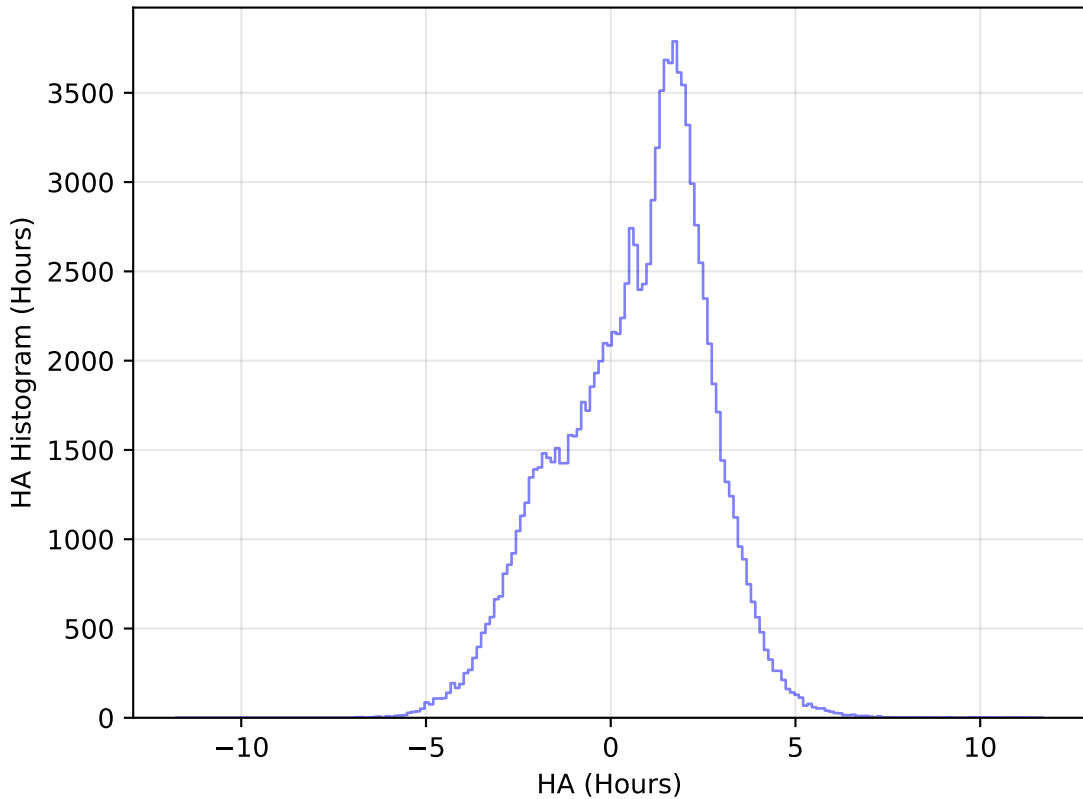
too_ignore_100_1v3.4_10yrs All sky u band: HA Histogram
