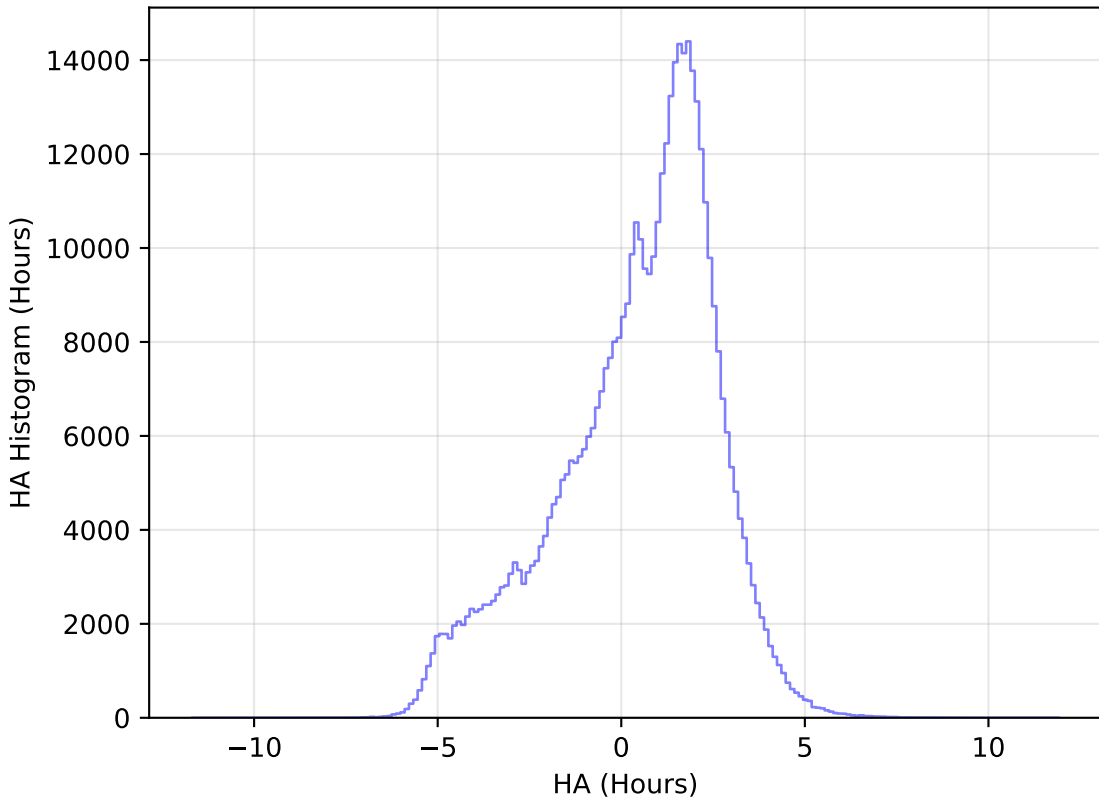
too_ignore_100_1v3.4_10yrs All sky r band: HA Histogram
