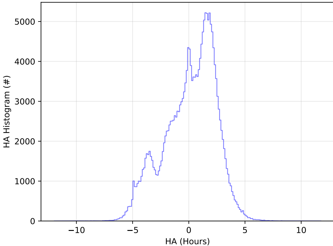
too_ignore_100_1v3.4_10yrs All sky g band: HA Histogram
