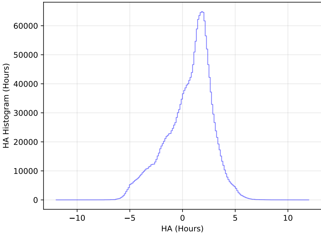
too_ignore_100_1v3.4_10yrs All sky all bands: HA Histogram
